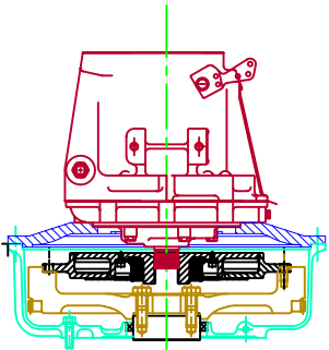
DETAIL OF FLYWHEEL AND MARINE GEAR ASSEMBLY SCALE 1:1
